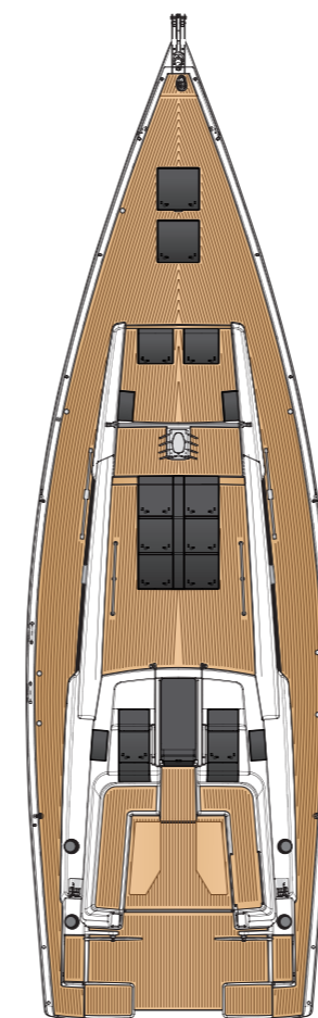
Beam 5.20 m | 17'1"
